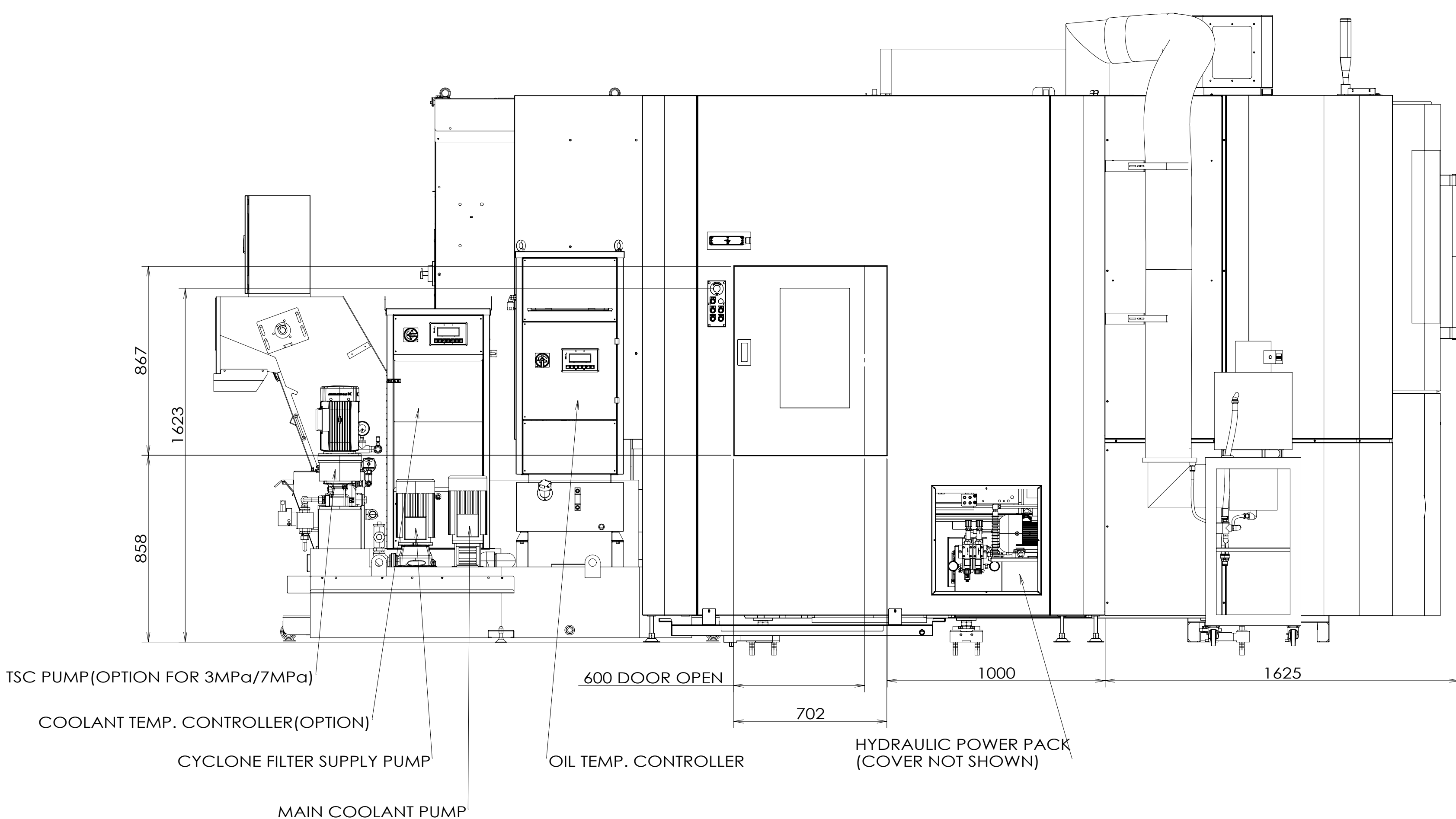
LEFT SIDE VIEW
